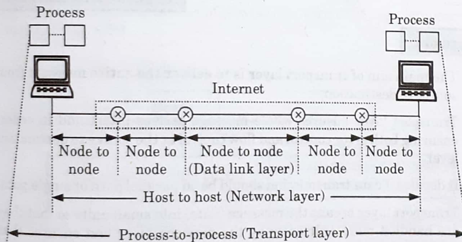
Fig. 4.1.1. Types of data deliveries.
