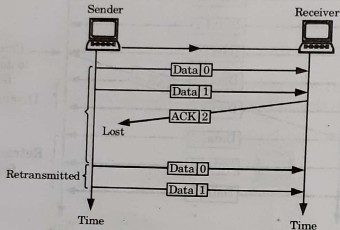
Fig. 2.25.3. Go-back-N, lost ACK frame.
