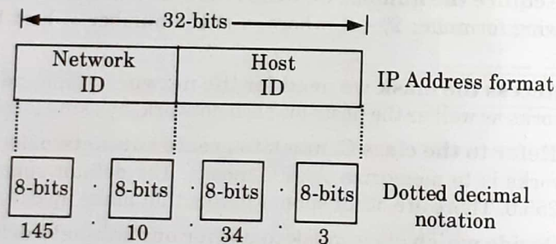
Fig. 3.21.2. IPv4 address format and dotted decimal format.
