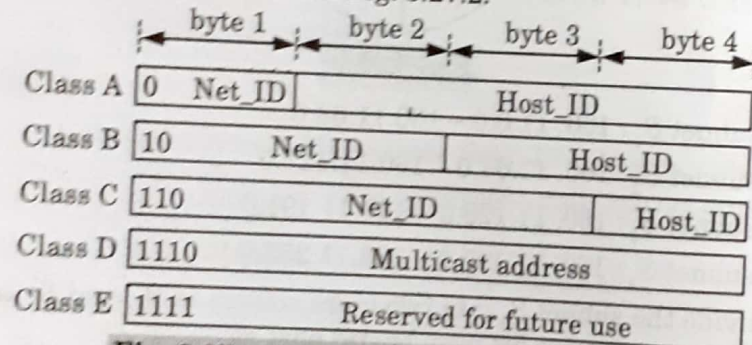
Fig. 3.27.1. Internet classes (IP addresses).
