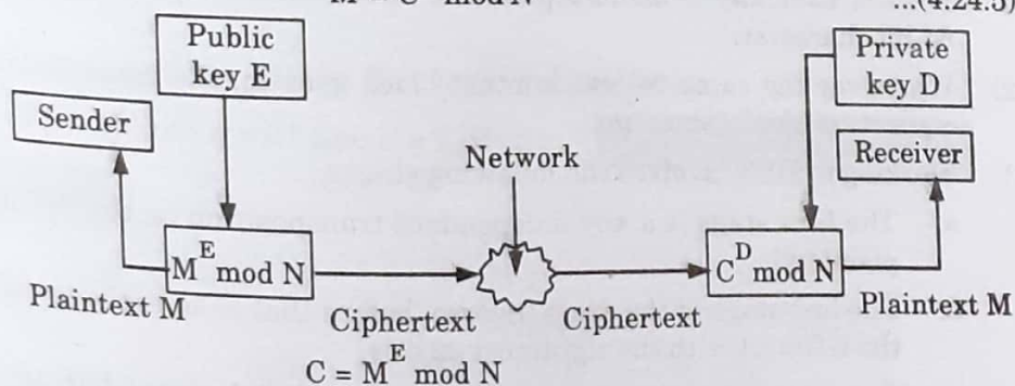
Fig. 4.24.1. Encryption and decryption in RSA.
