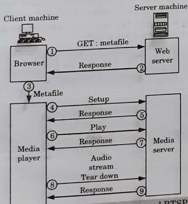
Fig. 4.19.4. Using a media server and RTSP.
