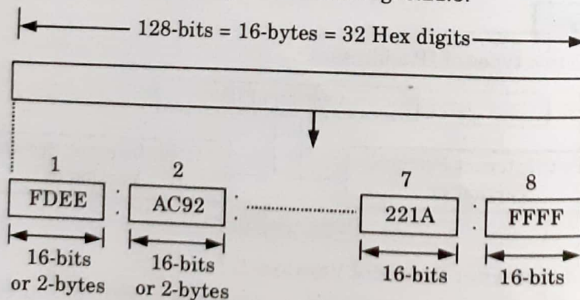
Fig. 3.21.3. IPv6 address.
