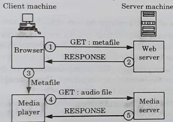
Fig. 4.19.3. Using a media server.
