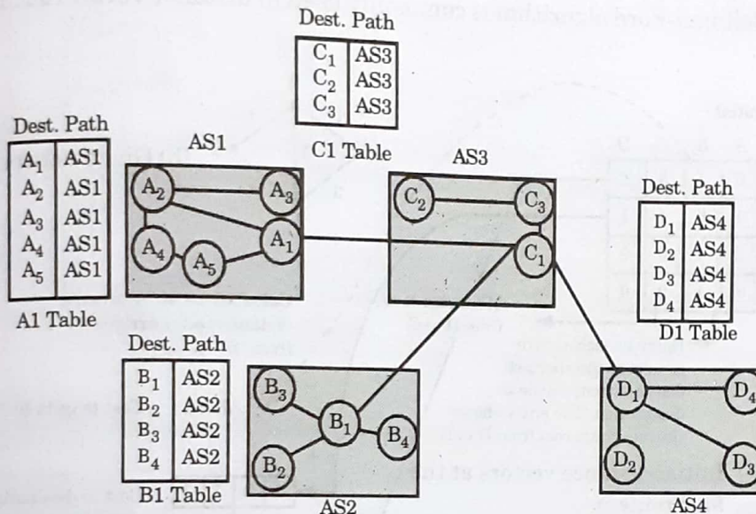
Fig. 3.6.1. Initial routing tables in path vector routing.
