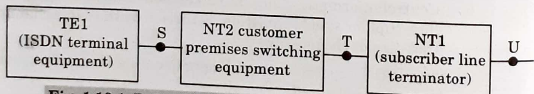
Fig. 1.19.1. Reference points and functional grouping in ISDN.
