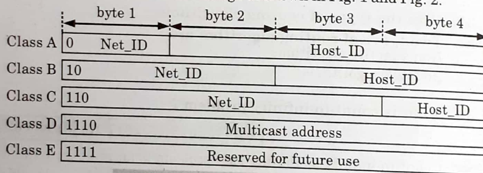
Fig. 3.6.1. Internet classes (IP addresses).
