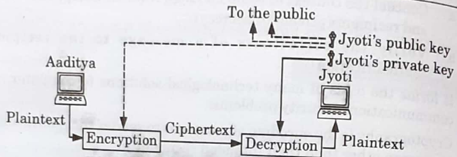
Fig. 4.22.2. Asymmetric key cryptography.
