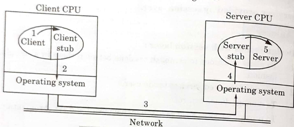
Fig. 4.14.1. Steps in making RPC.
