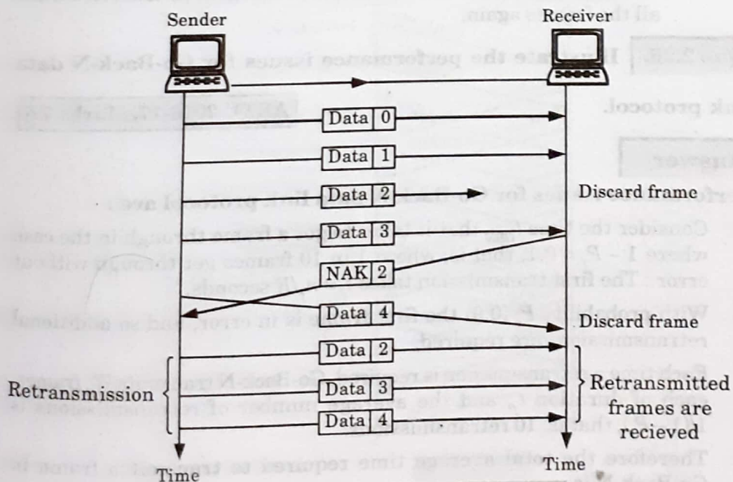
Fig. 2.25.2. Go-back-N, lost data frame.
