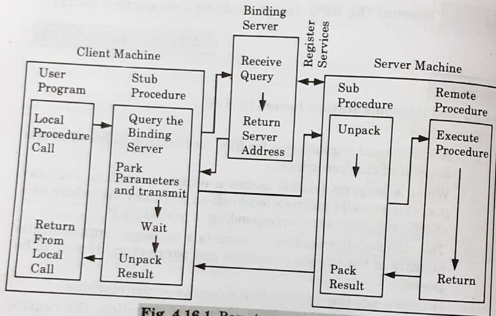
Fig. 4.16.1. Remote procedure call.
