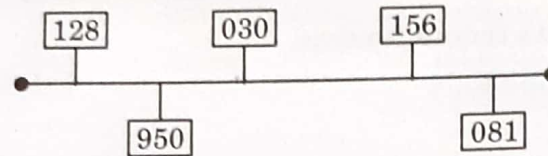
Fig. 2.16.1. Physical topology in token passing.
