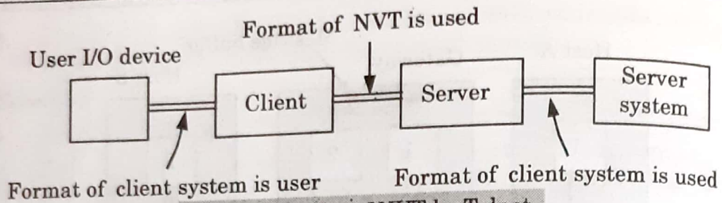
Fig. 5.11.1. Use of NVT by Telnet.
