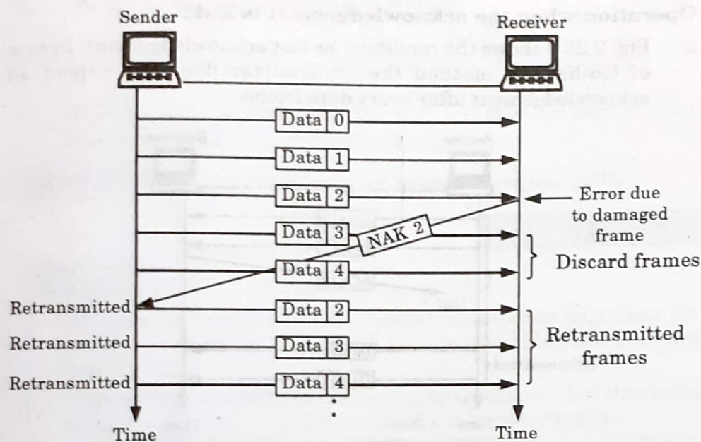
Fig. 2.25.1. Go-back-N, damaged data frame.
