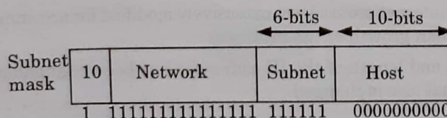
Fig. 3.24.1. One of the ways to subnet a class B network.
